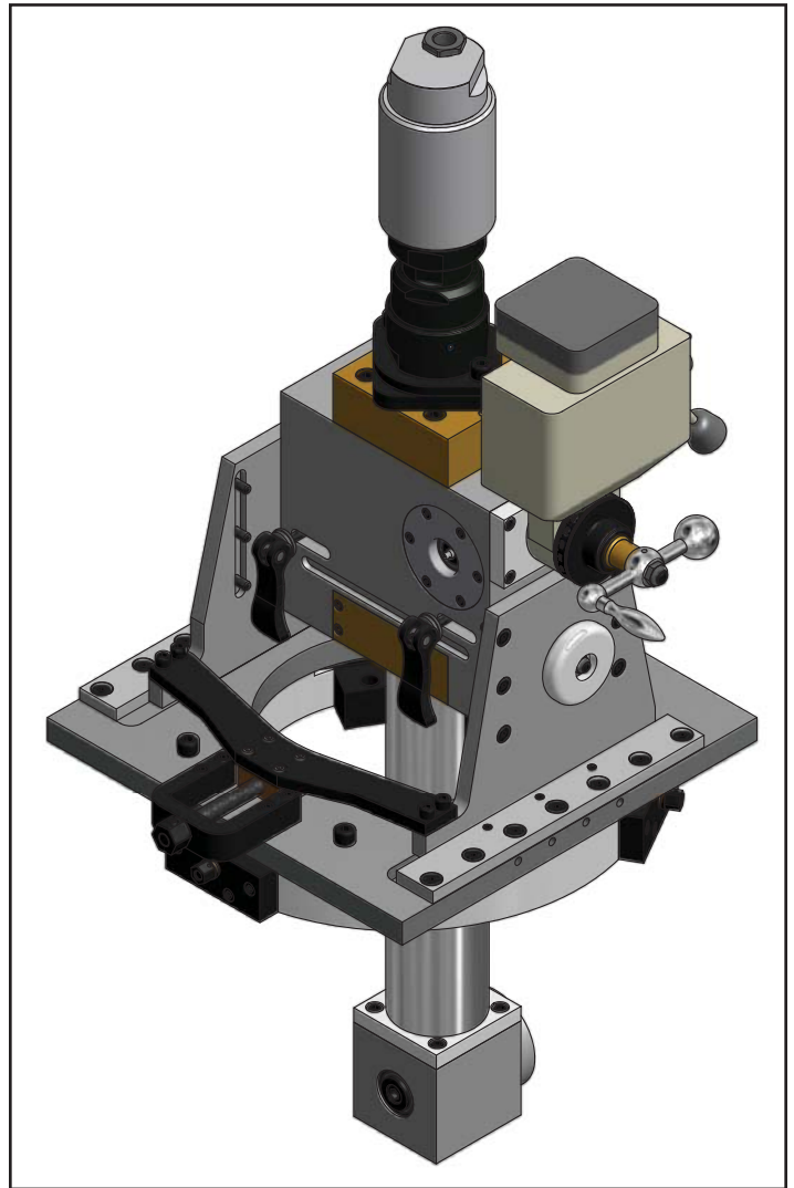
Flywheel Keyway Cutter
